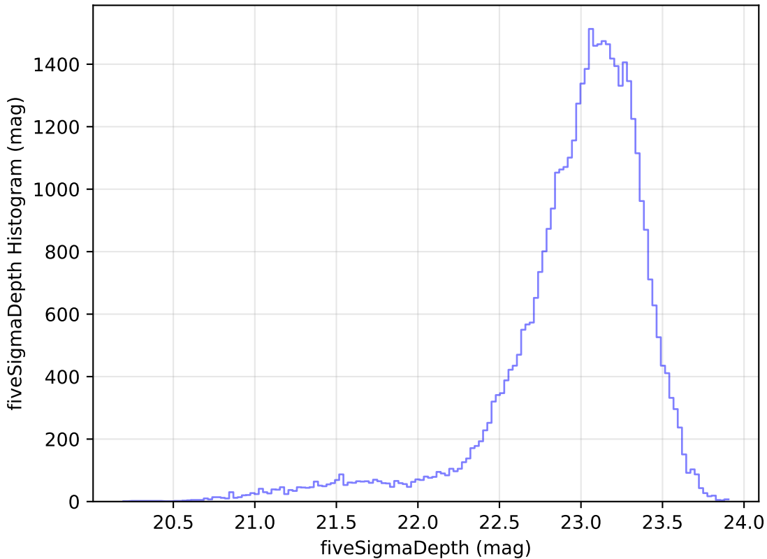
ddf_loaded_half_fl1_v3.4_10yrs Yr 1 z band: fiveSigmaDepth Histogram
