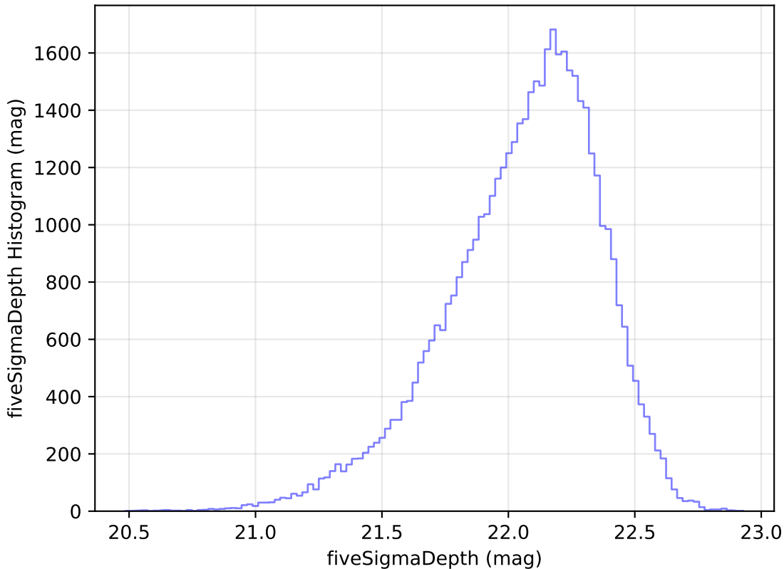
ddf_loaded_half_fl1_v3.4_10yrs Yr 1 y band: fiveSigmaDepth Histogram
