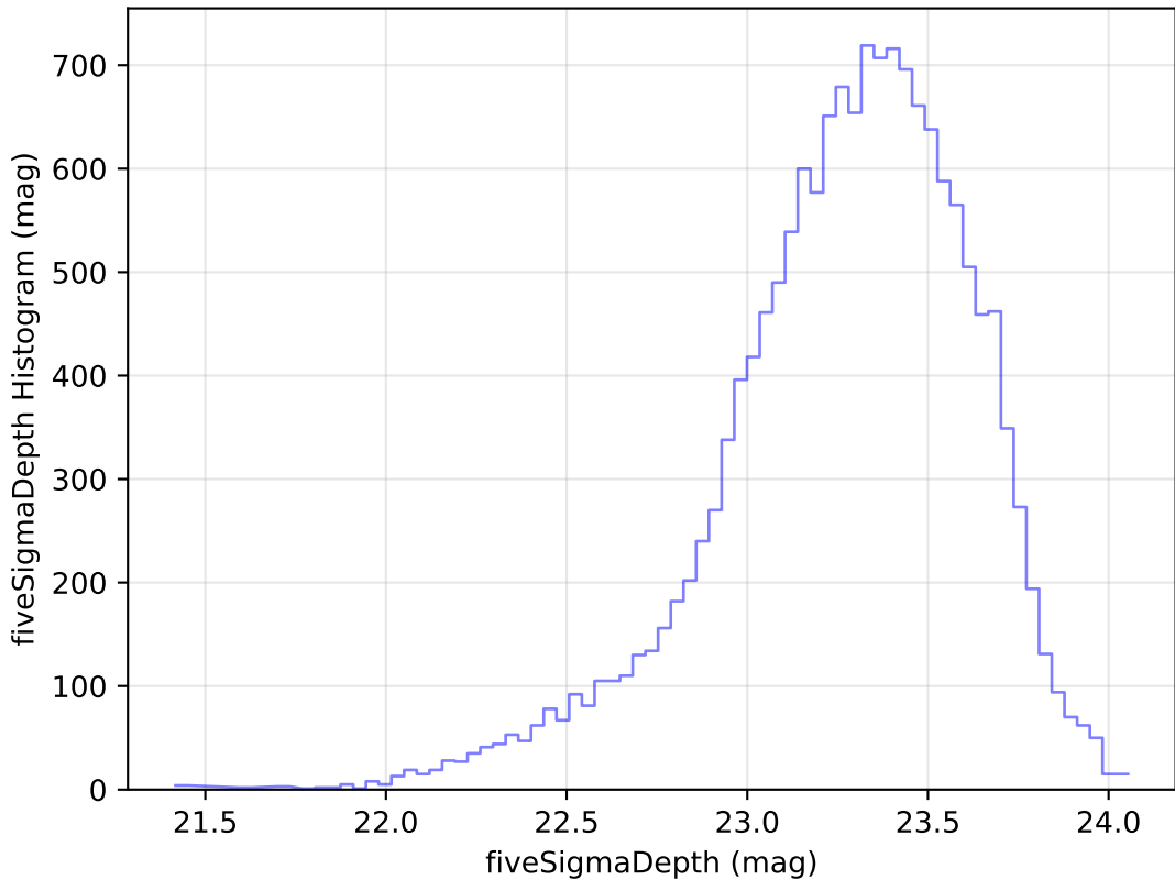
ddf_loaded_half_fl1_v3.4_10yrs Yr 1 u band: fiveSigmaDepth Histogram
