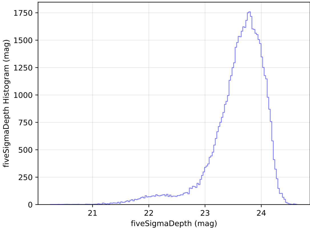
ddf_loaded_half_fl1_v3.4_10yrs Yr 1 i band: fiveSigmaDepth Histogram
