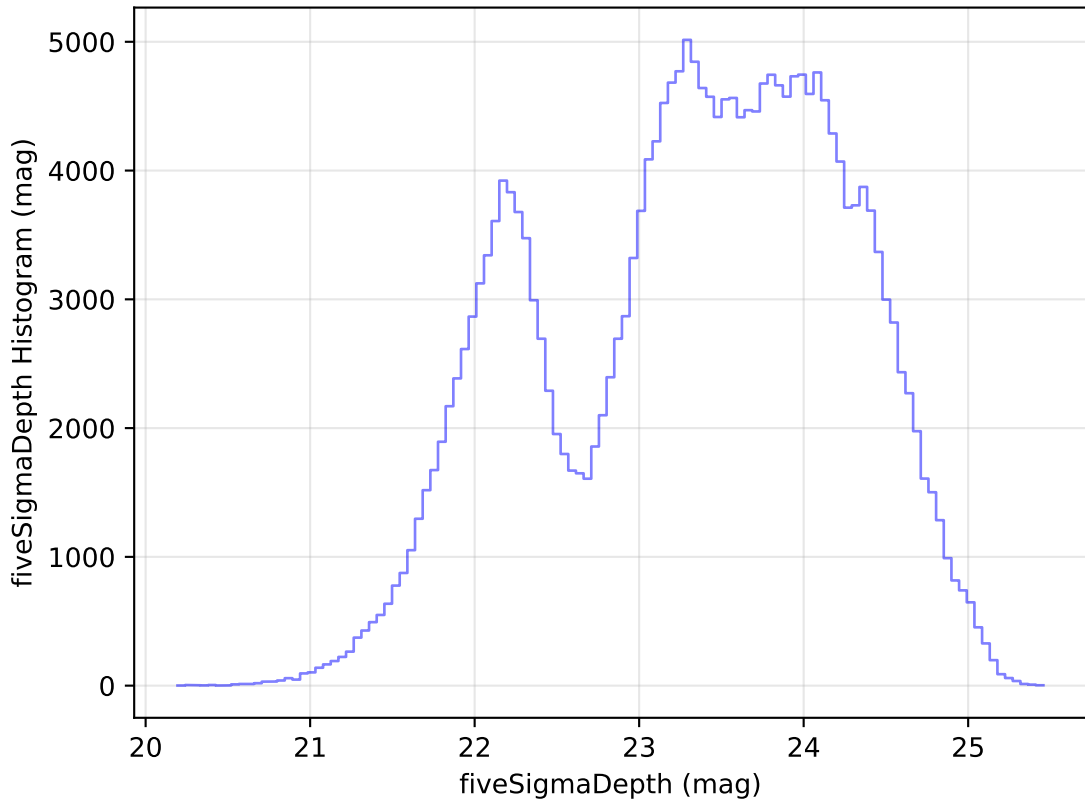
ddf_loaded_half_fl1_v3.4_10yrs Yr 1 all bands: fiveSigmaDepth Histogram
