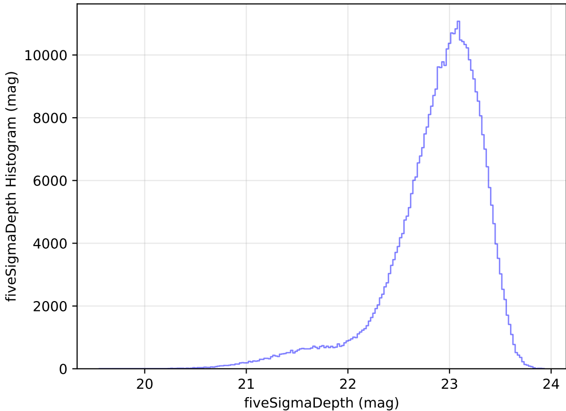
ddf_loaded_half_fl1_v3.4_10yrs WFD z band: fiveSigmaDepth Histogram
