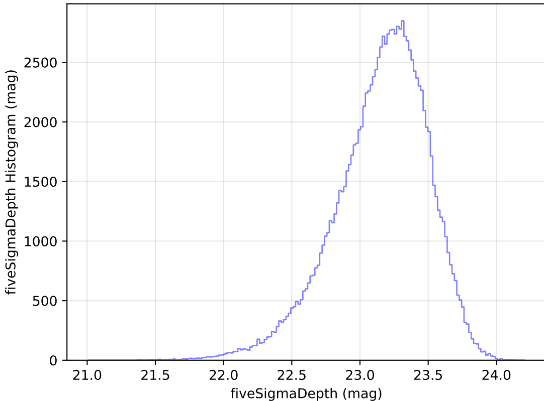
ddf_loaded_half_fl1_v3.4_10yrs WFD u band: fiveSigmaDepth Histogram
