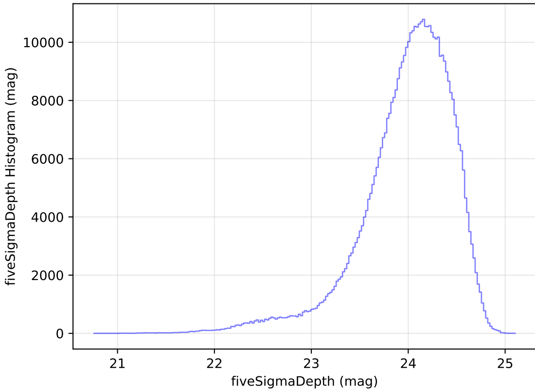
ddf_loaded_half_fl1_v3.4_10yrs WFD r band: fiveSigmaDepth Histogram
