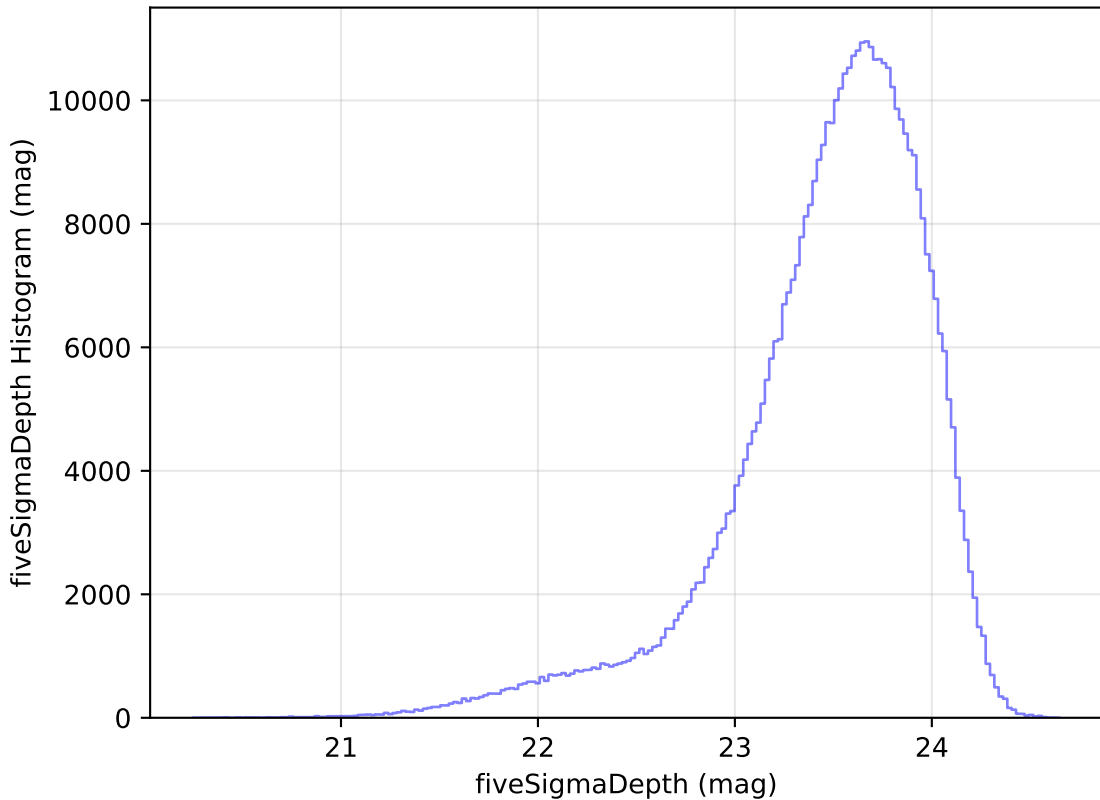
ddf_loaded_half_fl1_v3.4_10yrs WFD i band: fiveSigmaDepth Histogram
