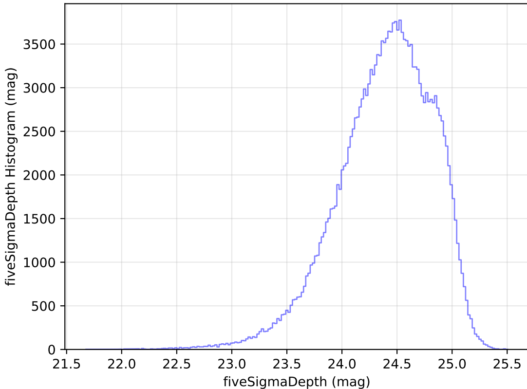
ddf_loaded_half_fl1_v3.4_10yrs WFD g band: fiveSigmaDepth Histogram
