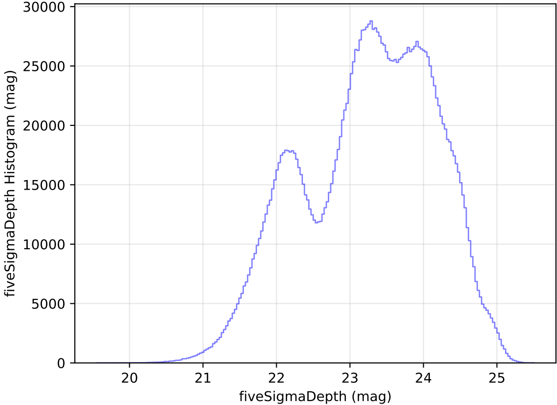
ddf_loaded_half_fl1_v3.4_10yrs WFD all bands: fiveSigmaDepth Histogram
