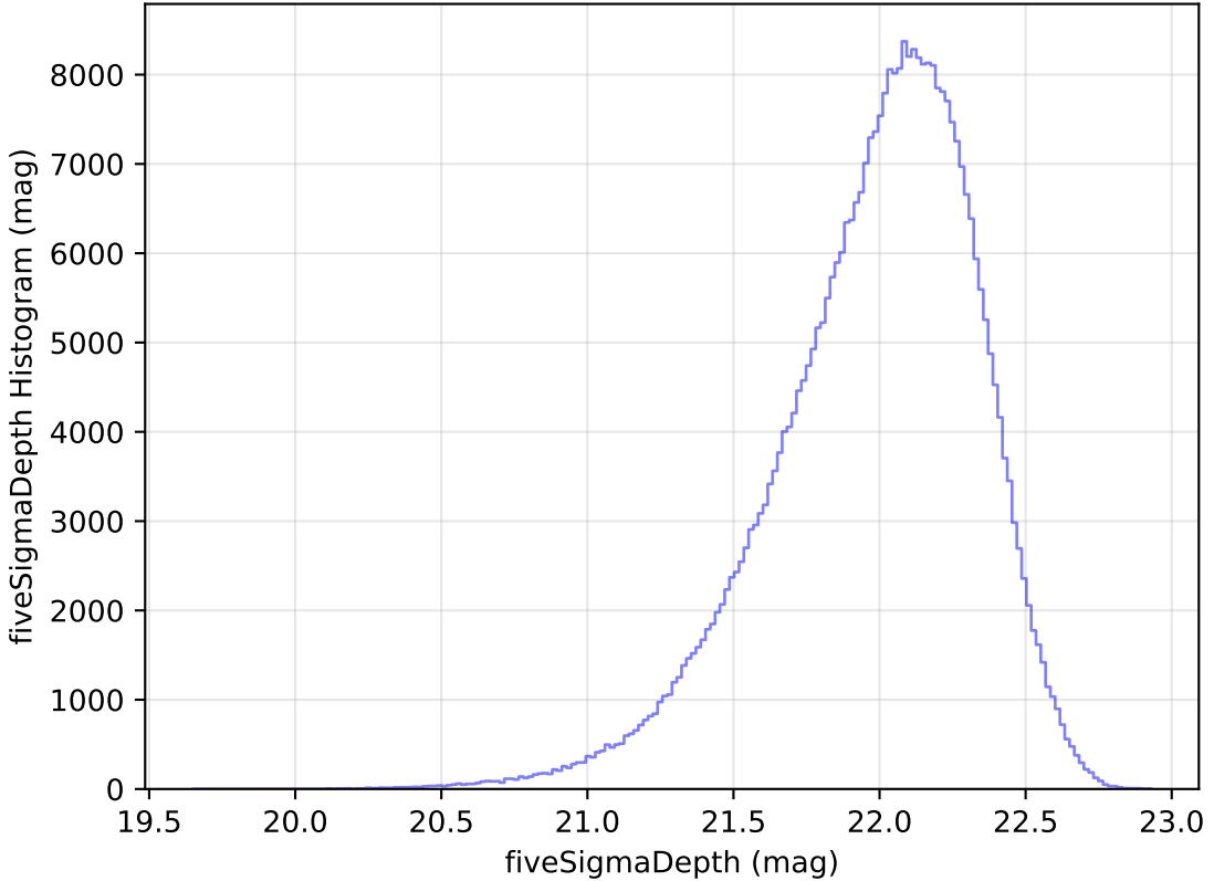
ddf_loaded_half_fl1_v3.4_10yrs All sky y band: fiveSigmaDepth Histogram
