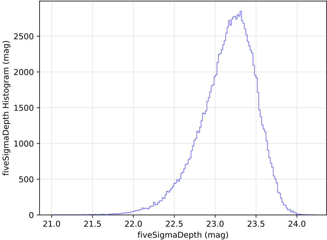
ddf_loaded_half_fl1_v3.4_10yrs All sky u band: fiveSigmaDepth Histogram
