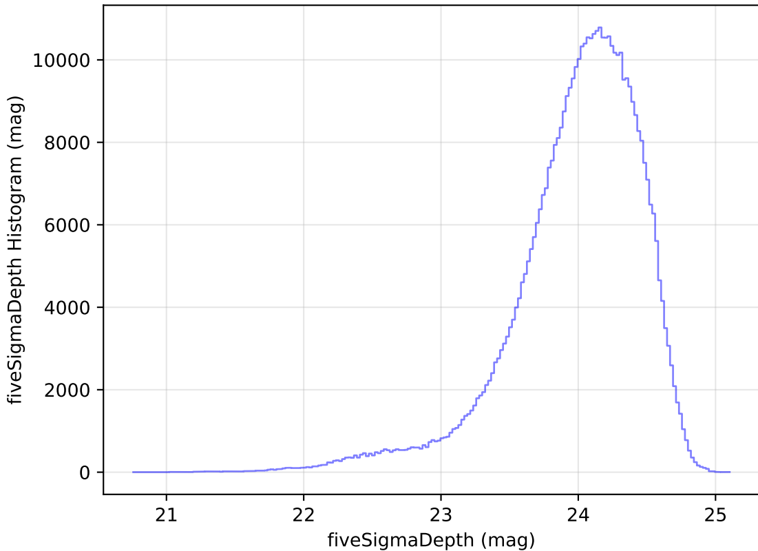
ddf_loaded_half_fl1_v3.4_10yrs All sky r band: fiveSigmaDepth Histogram
