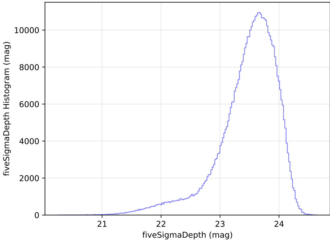
ddf_loaded_half_fl1_v3.4_10yrs All sky i band: fiveSigmaDepth Histogram
