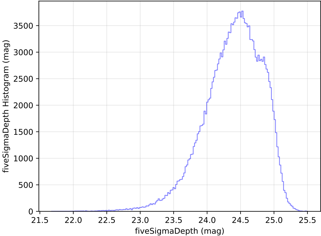
ddf_loaded_half_fl1_v3.4_10yrs All sky g band: fiveSigmaDepth Histogram
