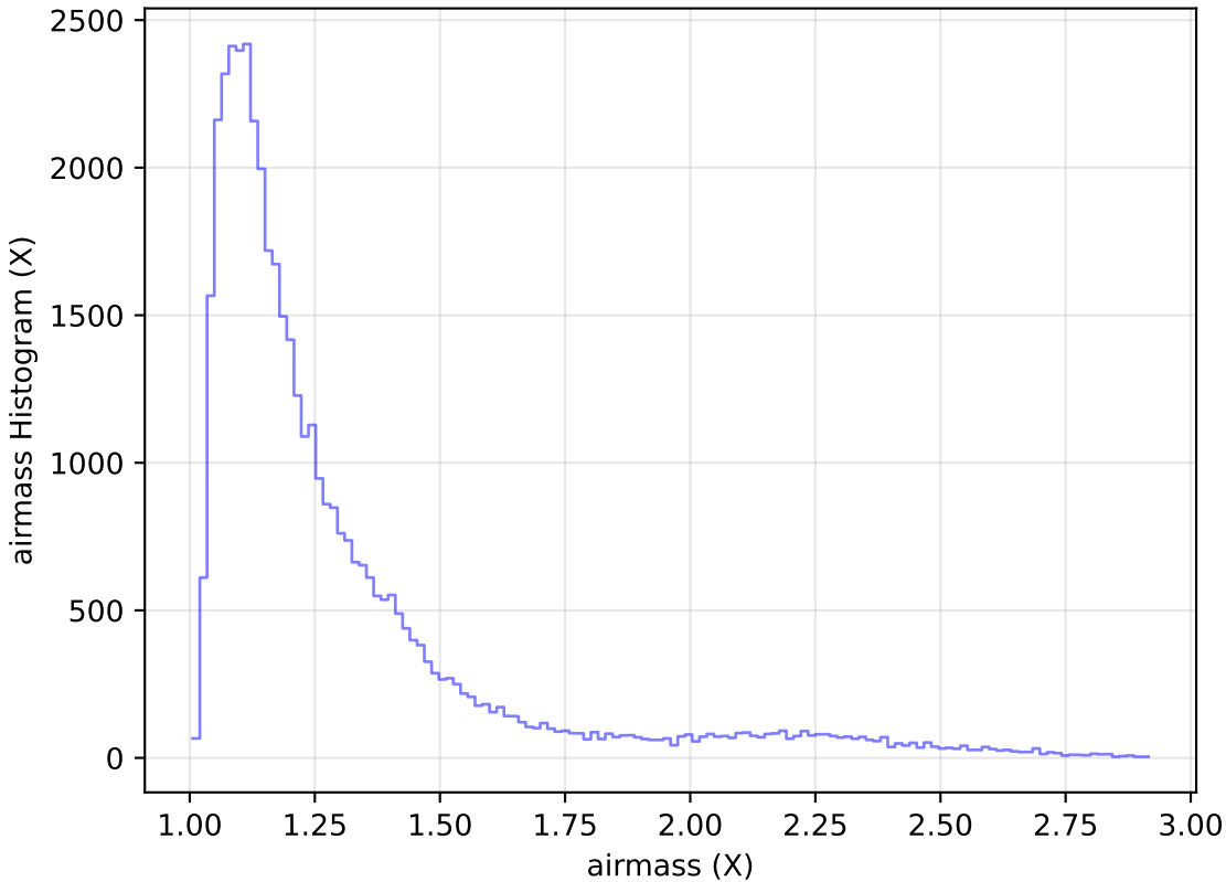
ddf_loaded_half_fl1_v3.4_10yrs Yr 1 z band: airmass Histogram
