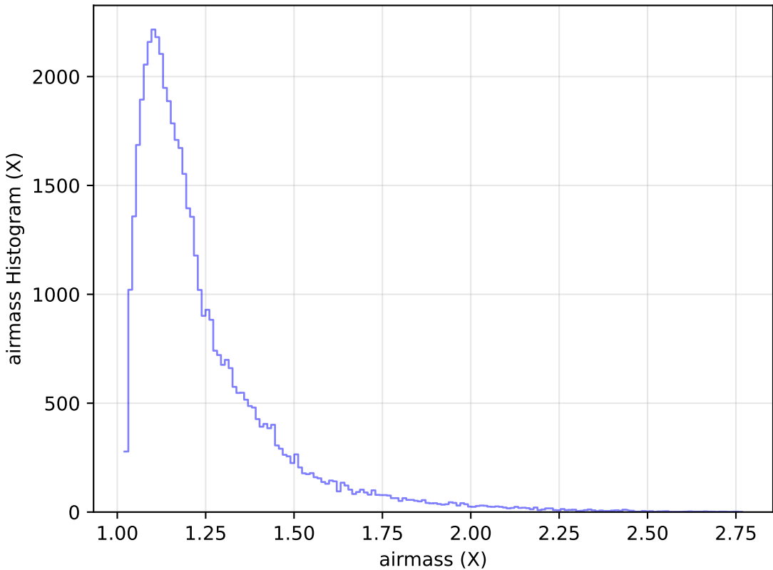
ddf_loaded_half_fl1_v3.4_10yrs Yr 1 y band: airmass Histogram
