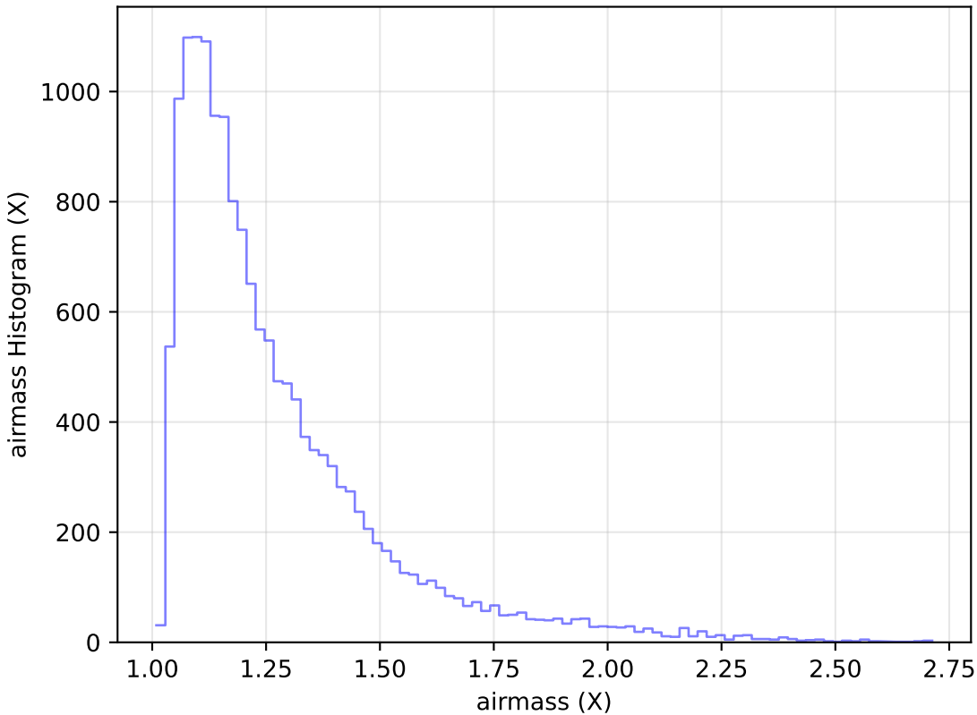
ddf_loaded_half_fl1_v3.4_10yrs Yr 1 u band: airmass Histogram
