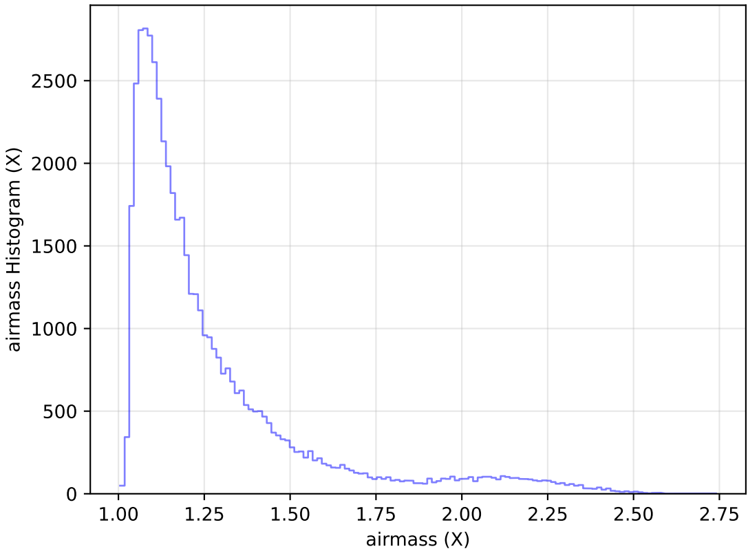
ddf_loaded_half_fl1_v3.4_10yrs Yr 1 r band: airmass Histogram
