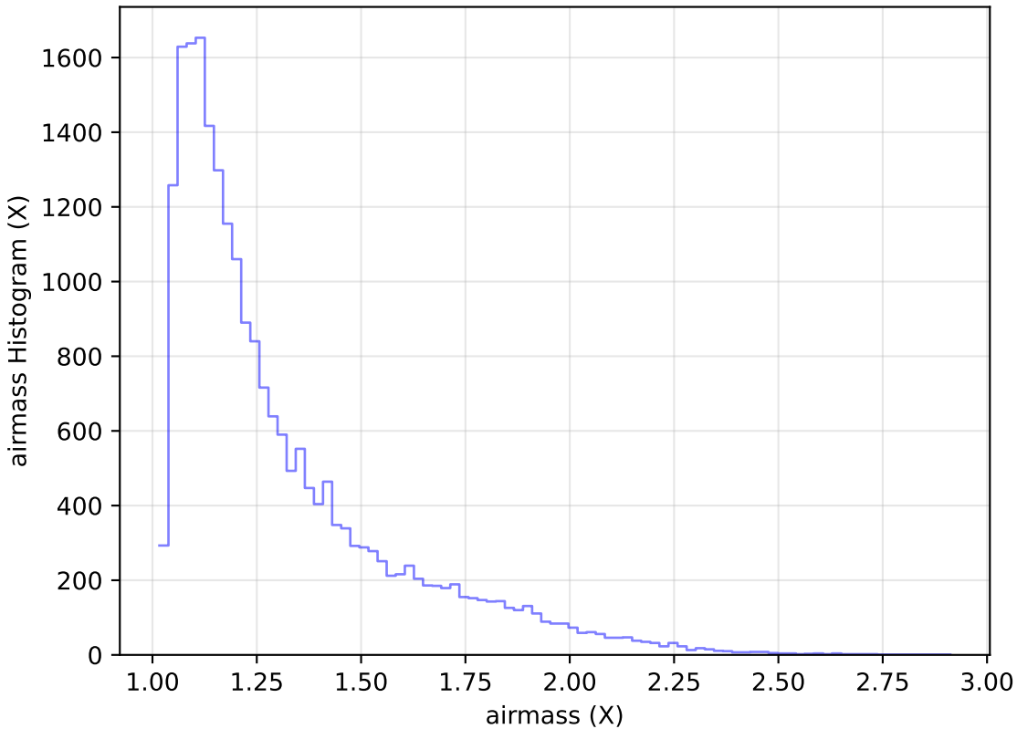
ddf_loaded_half_fl1_v3.4_10yrs Yr 1 g band: airmass Histogram
