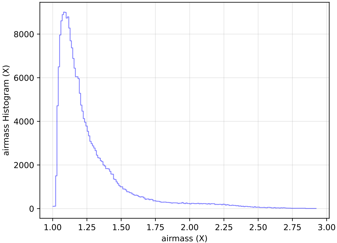
ddf_loaded_half_fl1_v3.4_10yrs Yr 1 all bands: airmass Histogram
