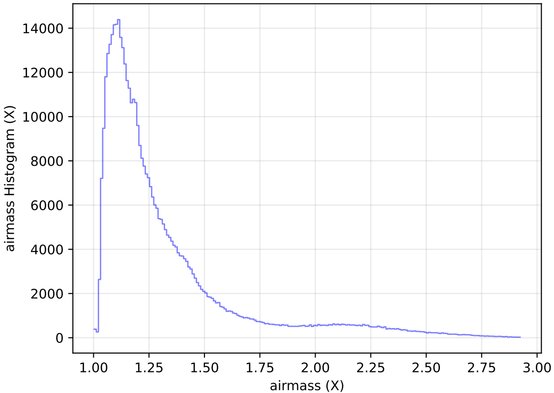
ddf_loaded_half_fl1_v3.4_10yrs WFD z band: airmass Histogram
