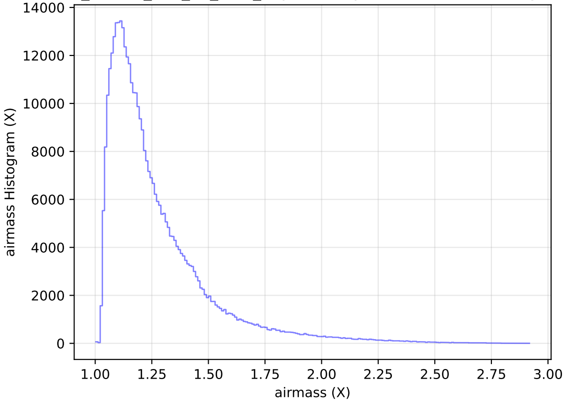
ddf_loaded_half_fl1_v3.4_10yrs WFD y band: airmass Histogram
