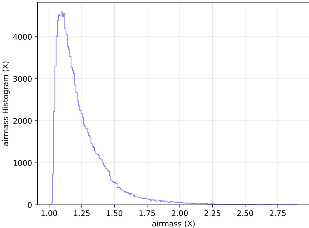
ddf_loaded_half_fl1_v3.4_10yrs WFD u band: airmass Histogram
