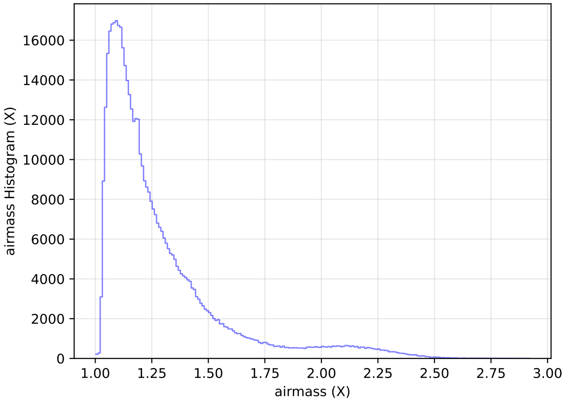
ddf_loaded_half_fl1_v3.4_10yrs WFD r band: airmass Histogram
