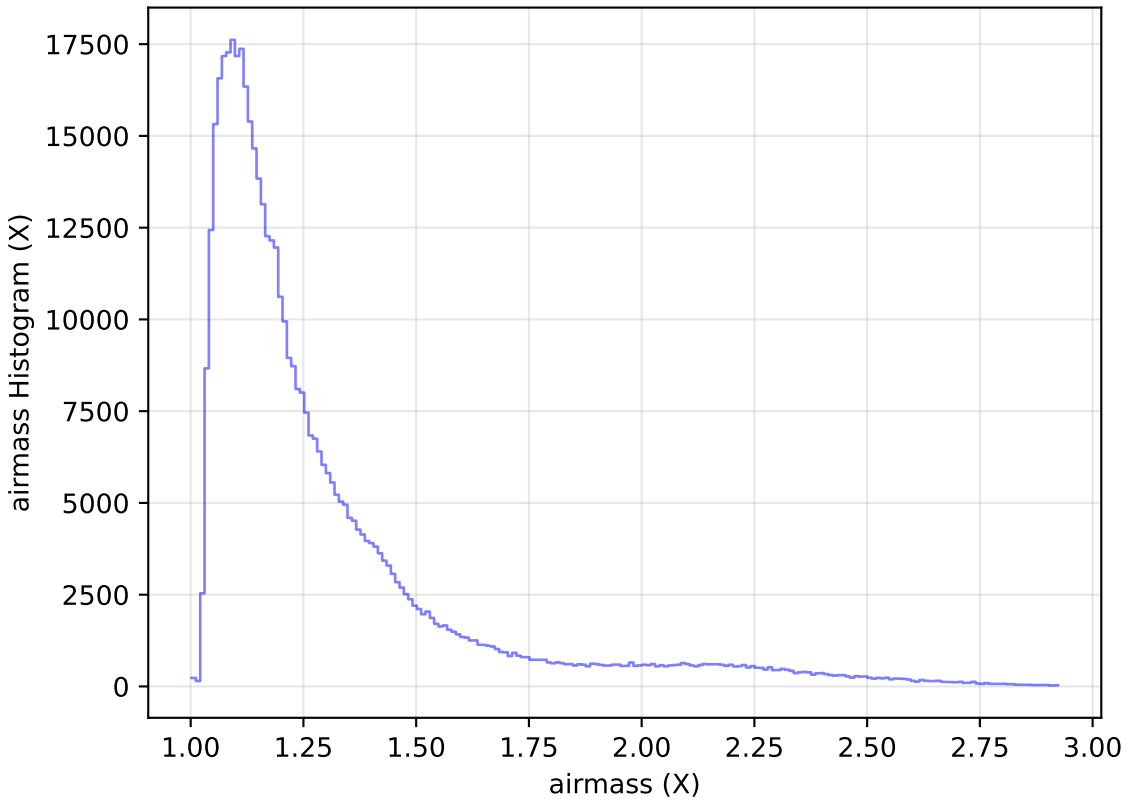
ddf_loaded_half_fl1_v3.4_10yrs WFD i band: airmass Histogram
