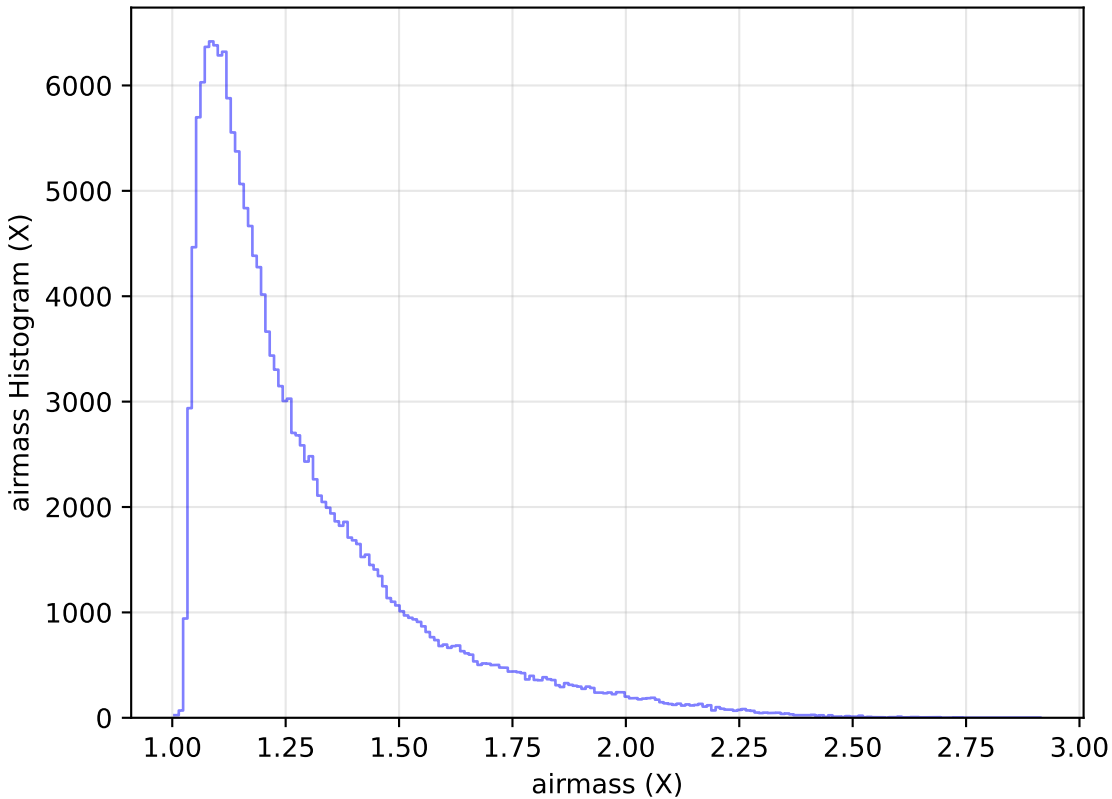
ddf_loaded_half_fl1_v3.4_10yrs WFD g band: airmass Histogram
