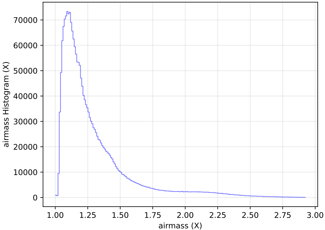
ddf_loaded_half_fl1_v3.4_10yrs WFD all bands: airmass Histogram
