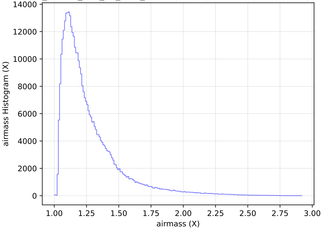
ddf_loaded_half_fl1_v3.4_10yrs All sky y band: airmass Histogram
