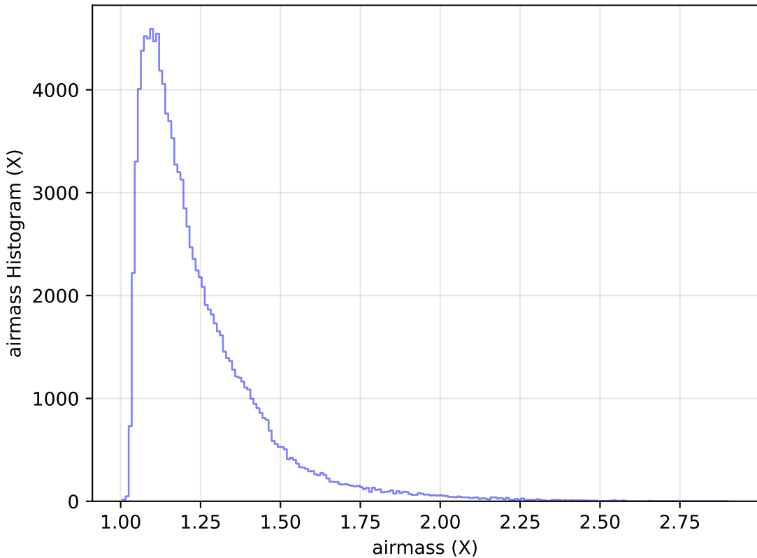
ddf_loaded_half_fl1_v3.4_10yrs All sky u band: airmass Histogram
