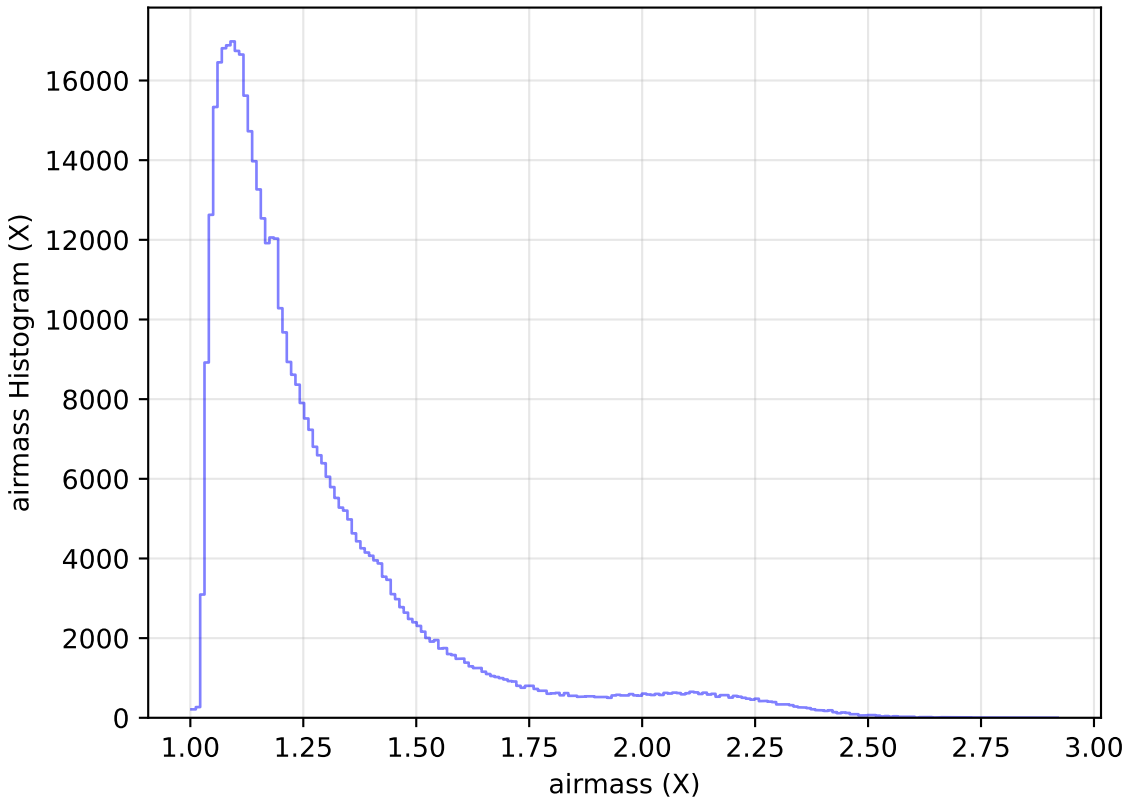
ddf_loaded_half_fl1_v3.4_10yrs All sky r band: airmass Histogram
