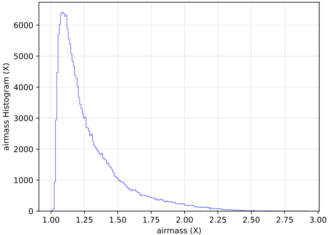
ddf_loaded_half_fl1_v3.4_10yrs All sky g band: airmass Histogram
