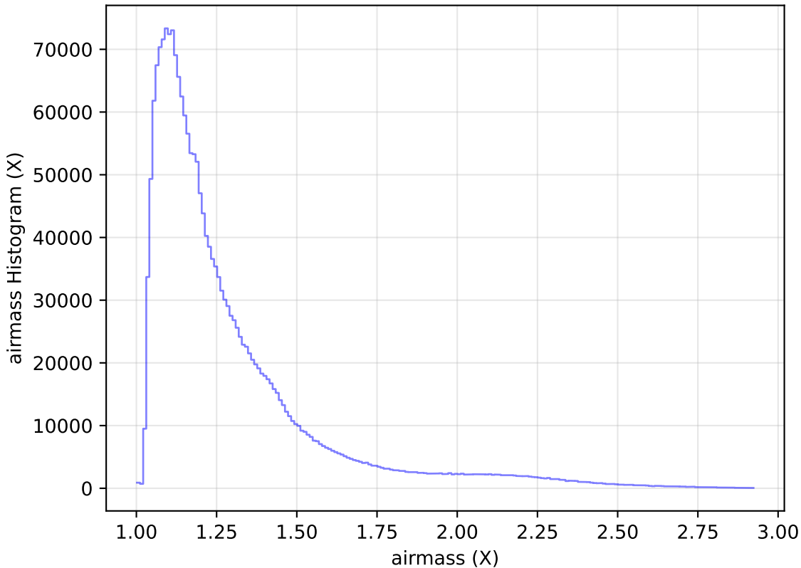
ddf_loaded_half_fl1_v3.4_10yrs All sky all bands: airmass Histogram
