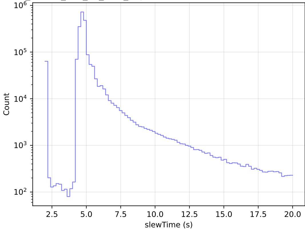
ddf_loaded_half_fl1_v3.4_10yrs All visits: Zoom Slew Time Histogram
