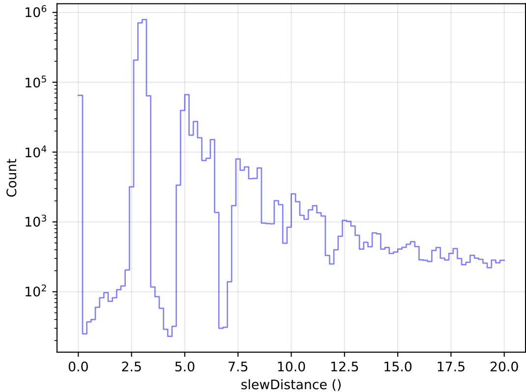
ddf_loaded_half_fl1_v3.4_10yrs All visits: Zoom Slew Distance Histogram
