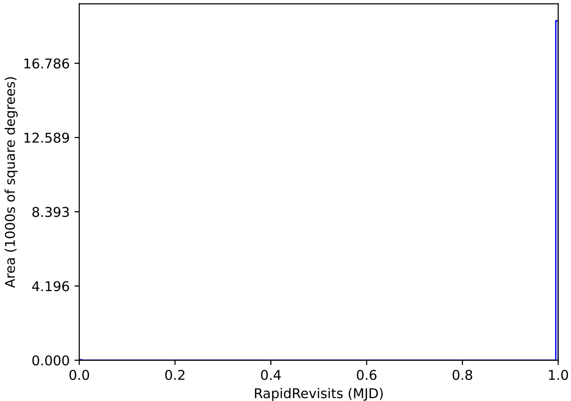
ddf_loaded_half_fl1_v3.4_10yrs WFD: RapidRevisits
