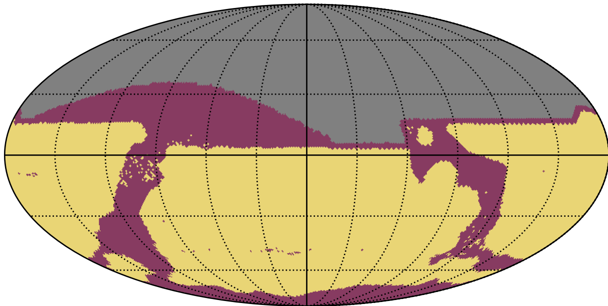
ddf_loaded_half_fl1_v3.4_10yrs All sky: RapidRevisits
