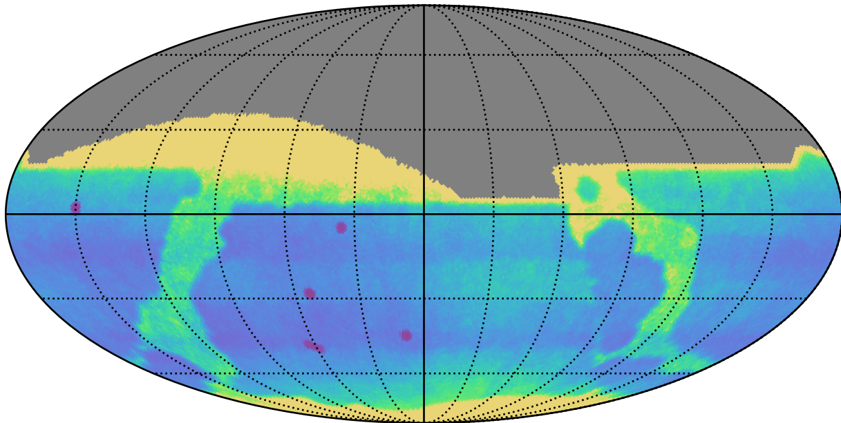
ddf_loaded_half_fl1_v3.4_10yrs All sky: Proper Motion Uncert @ 24.0
