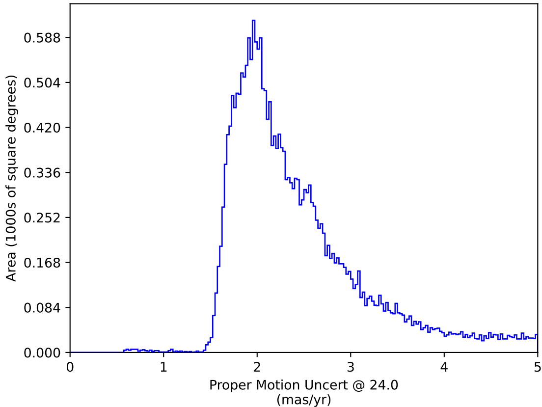
ddf_loaded_half_fl1_v3.4_10yrs All sky: Proper Motion Uncert @ 24.0
