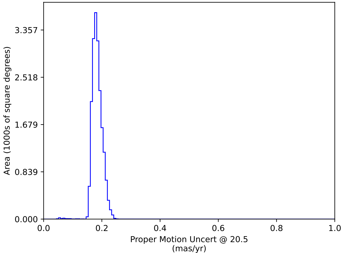
ddf_loaded_half_fl1_v3.4_10yrs WFD: Proper Motion Uncert @ 20.5
