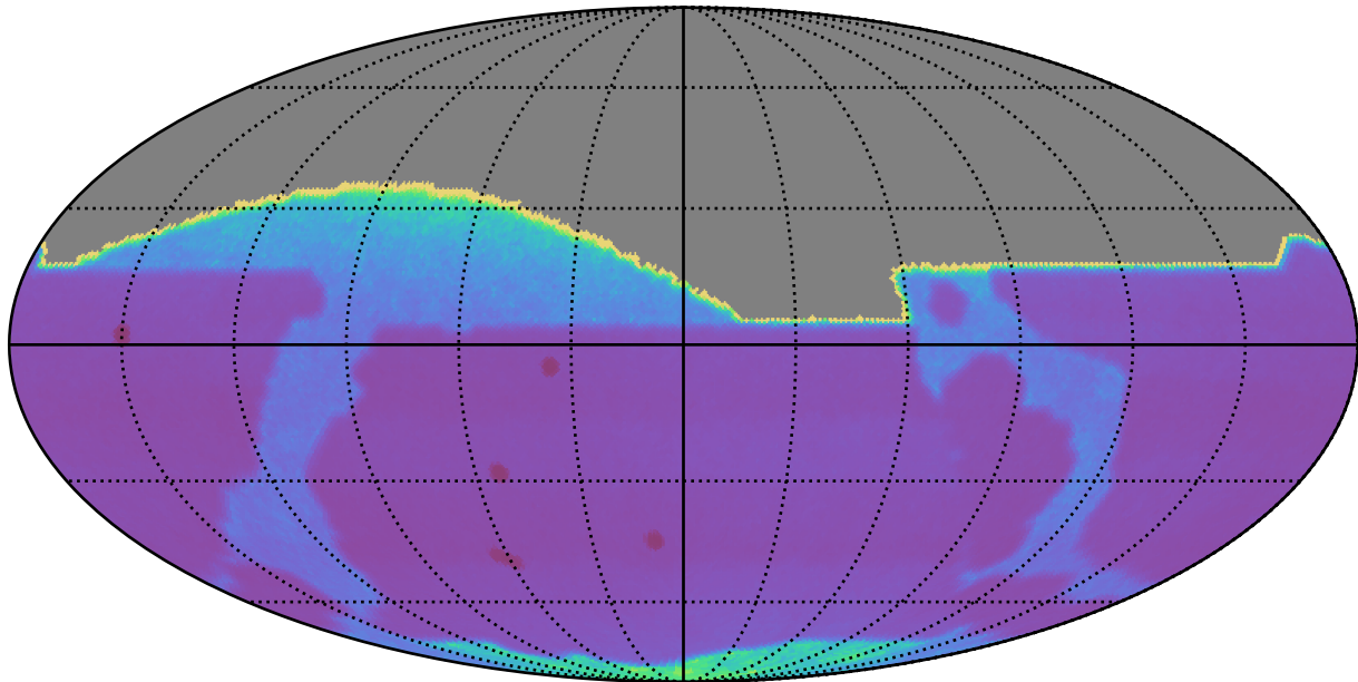
ddf_loaded_half_fl1_v3.4_10yrs All sky: Proper Motion Uncert @ 20.5
