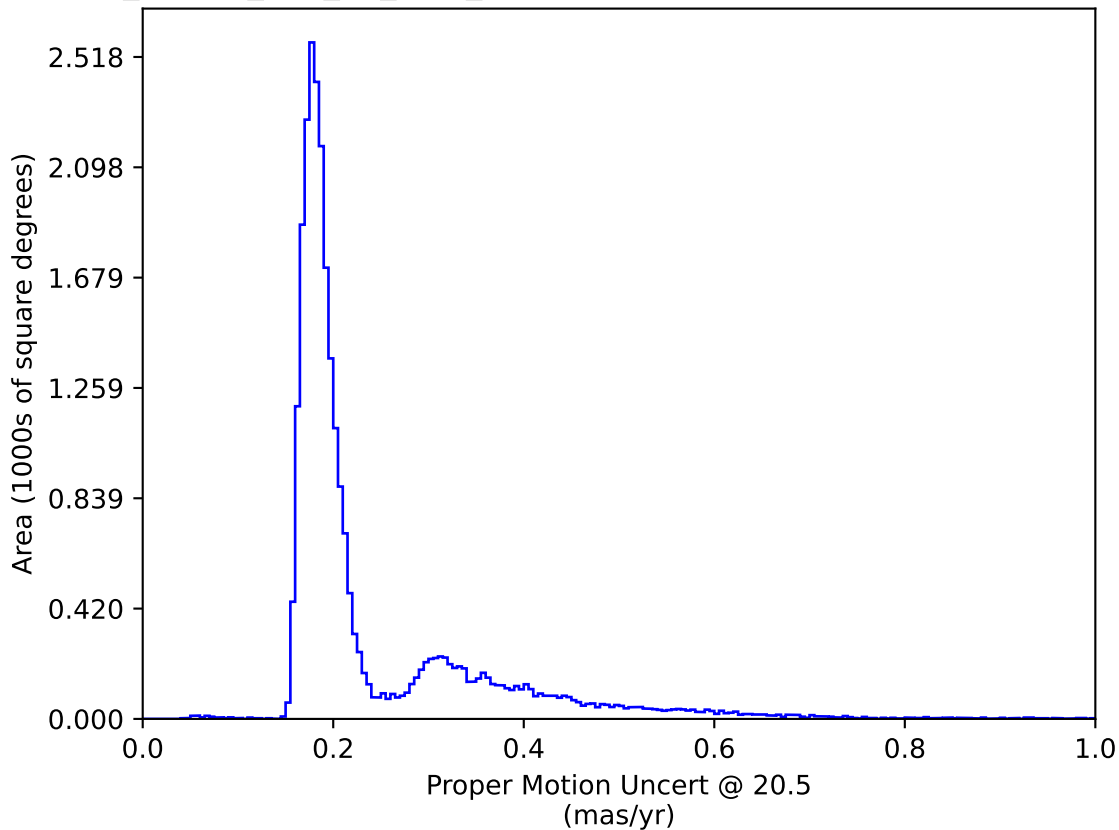
ddf_loaded_half_fl1_v3.4_10yrs All sky: Proper Motion Uncert @ 20.5
