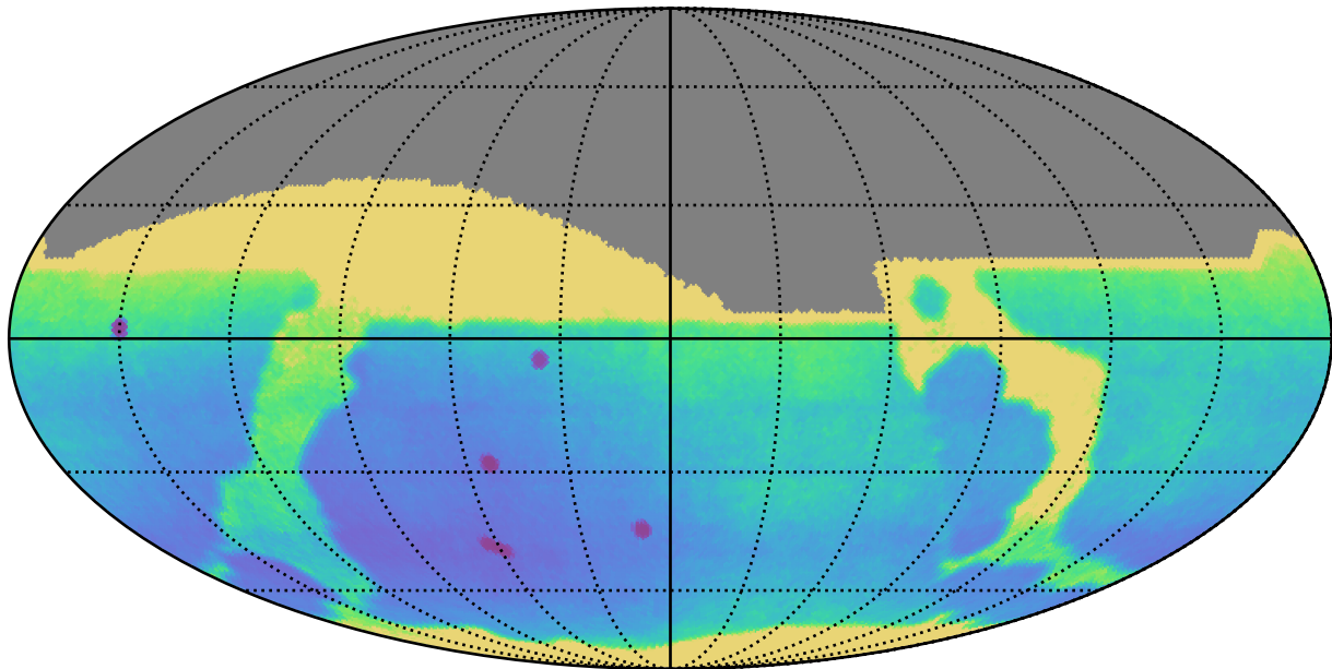
ddf_loaded_half_fl1_v3.4_10yrs All sky: Parallax Uncert @ 24.0
