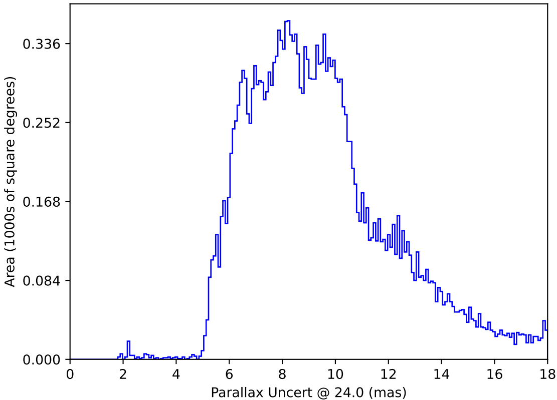
ddf_loaded_half_fl1_v3.4_10yrs All sky: Parallax Uncert @ 24.0
