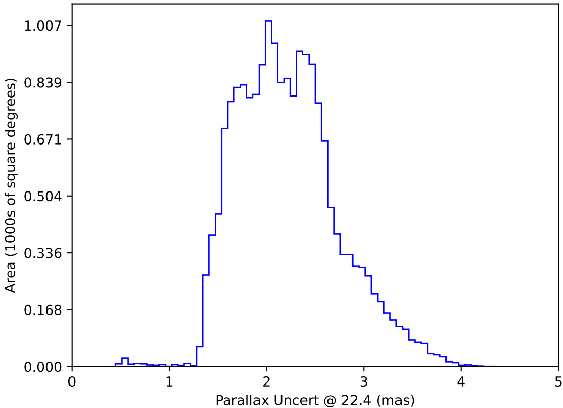
ddf_loaded_half_fl1_v3.4_10yrs WFD: Parallax Uncert @ 22.4
