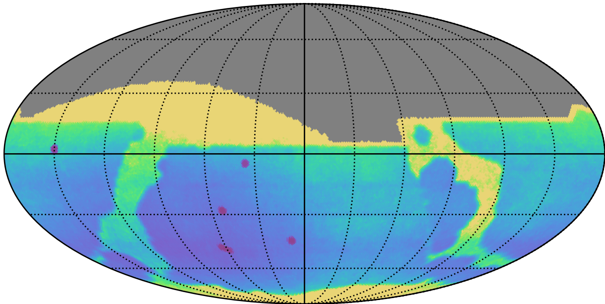
ddf_loaded_half_fl1_v3.4_10yrs All sky: Parallax Uncert @ 22.4
