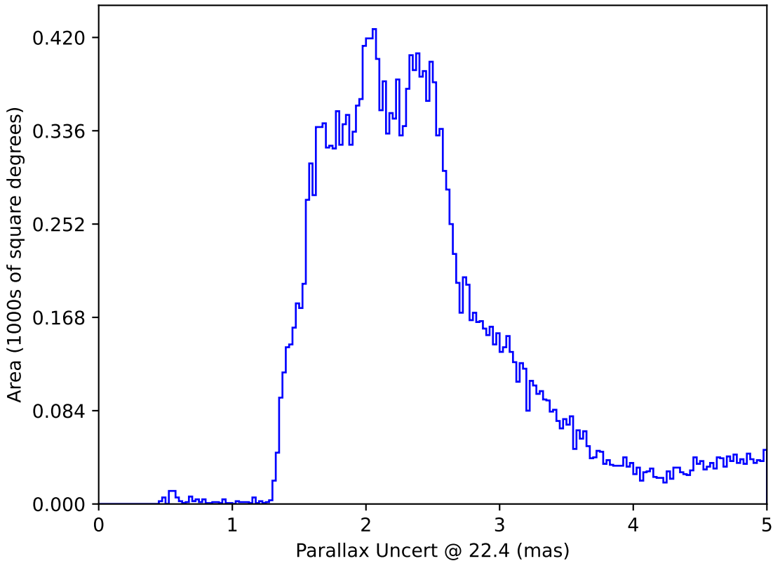
ddf_loaded_half_fl1_v3.4_10yrs All sky: Parallax Uncert @ 22.4
