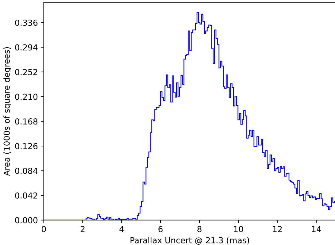
ddf_loaded_half_fl1_v3.4_10yrs All sky y band only: Parallax Uncert @ 21.3
