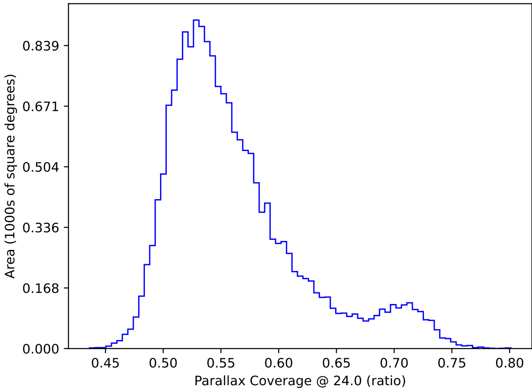
ddf_loaded_half_fl1_v3.4_10yrs WFD: Parallax Coverage @ 24.0
